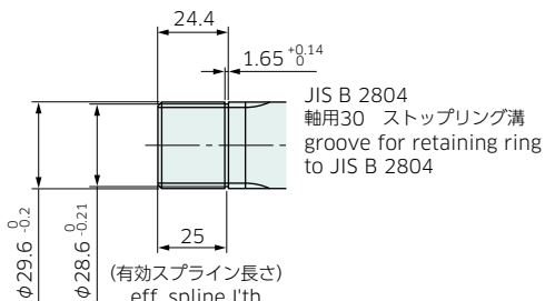
軸端詳細 detail of shaft end
